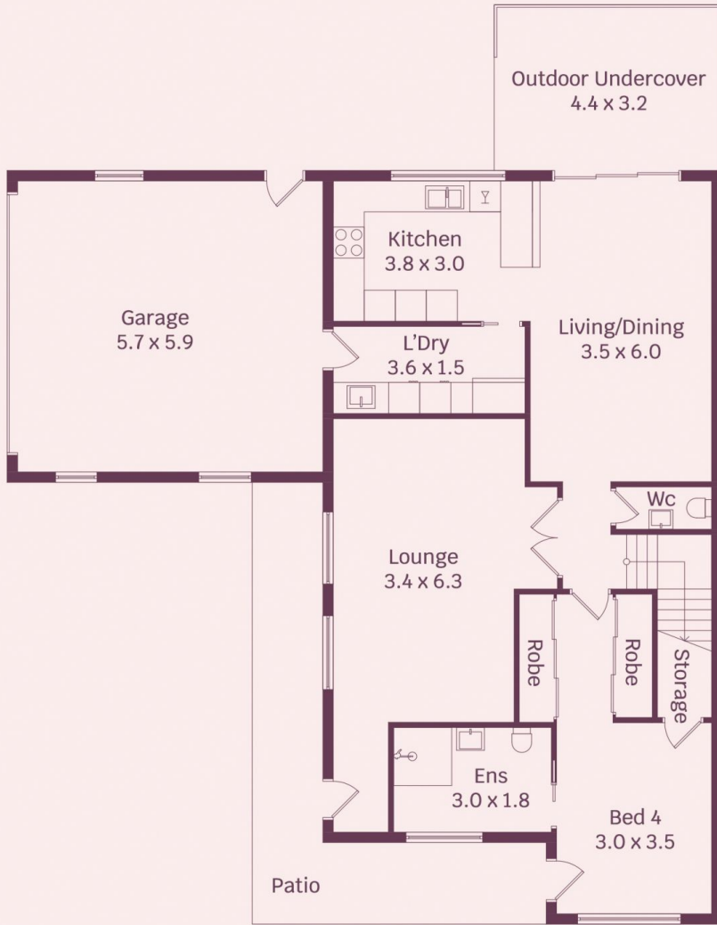
Ground Floor
