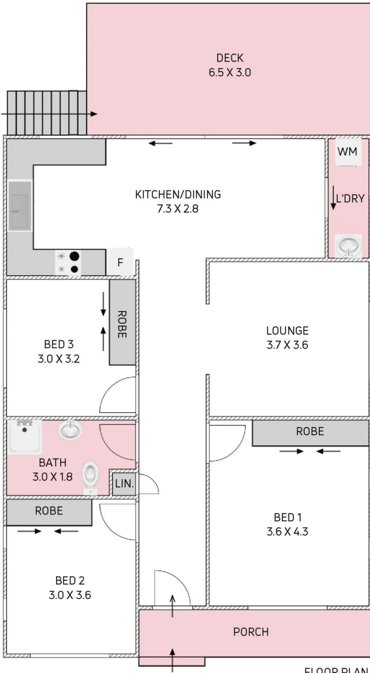
FLOOR PLAN
