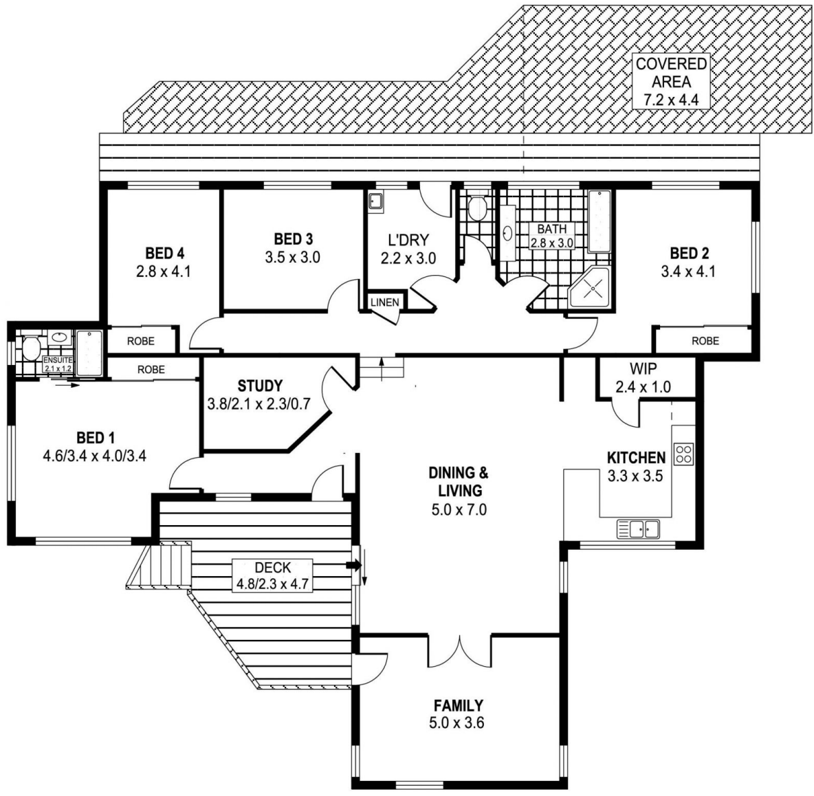
UPPER LEVEL
