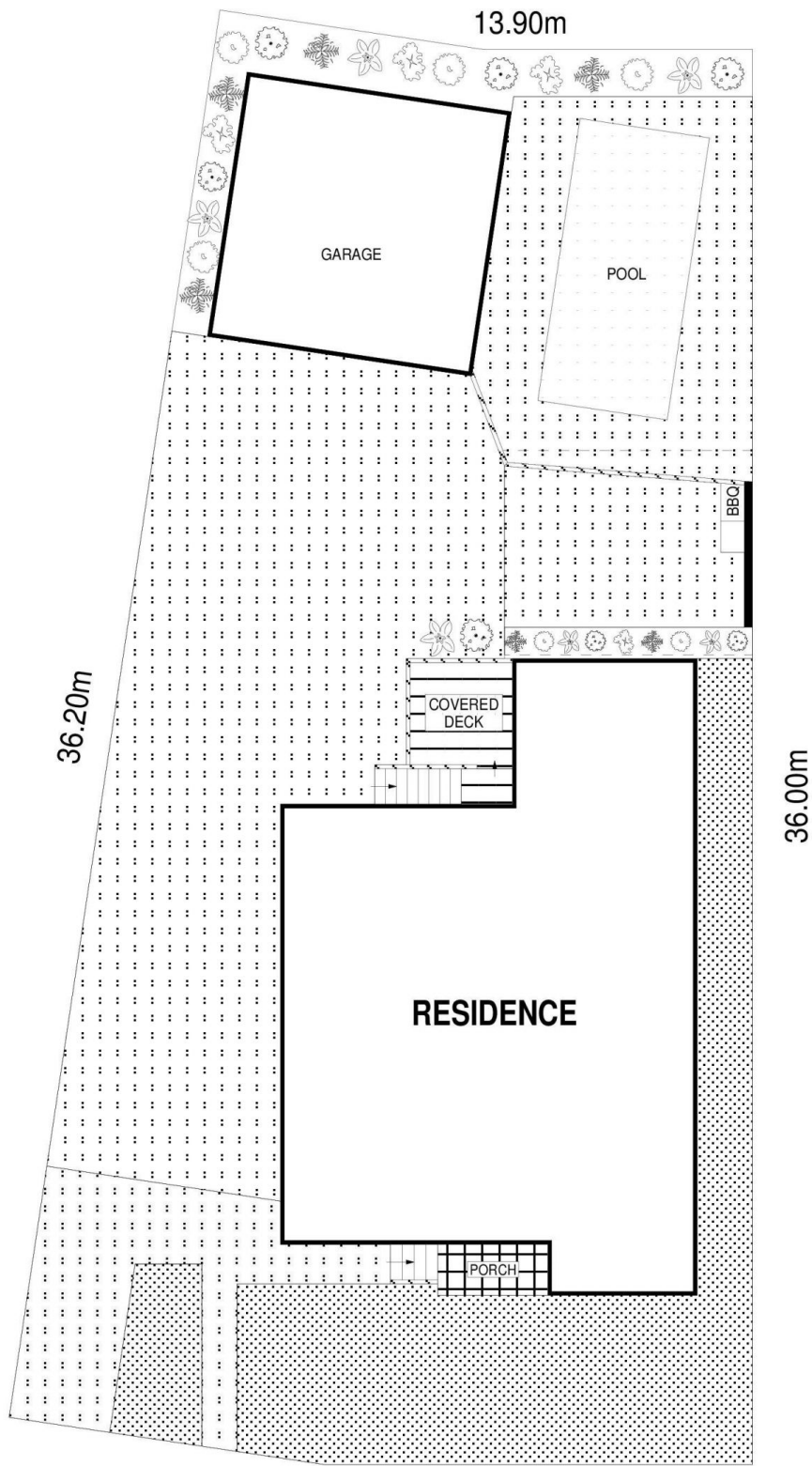
19.30m SITE PLAN
