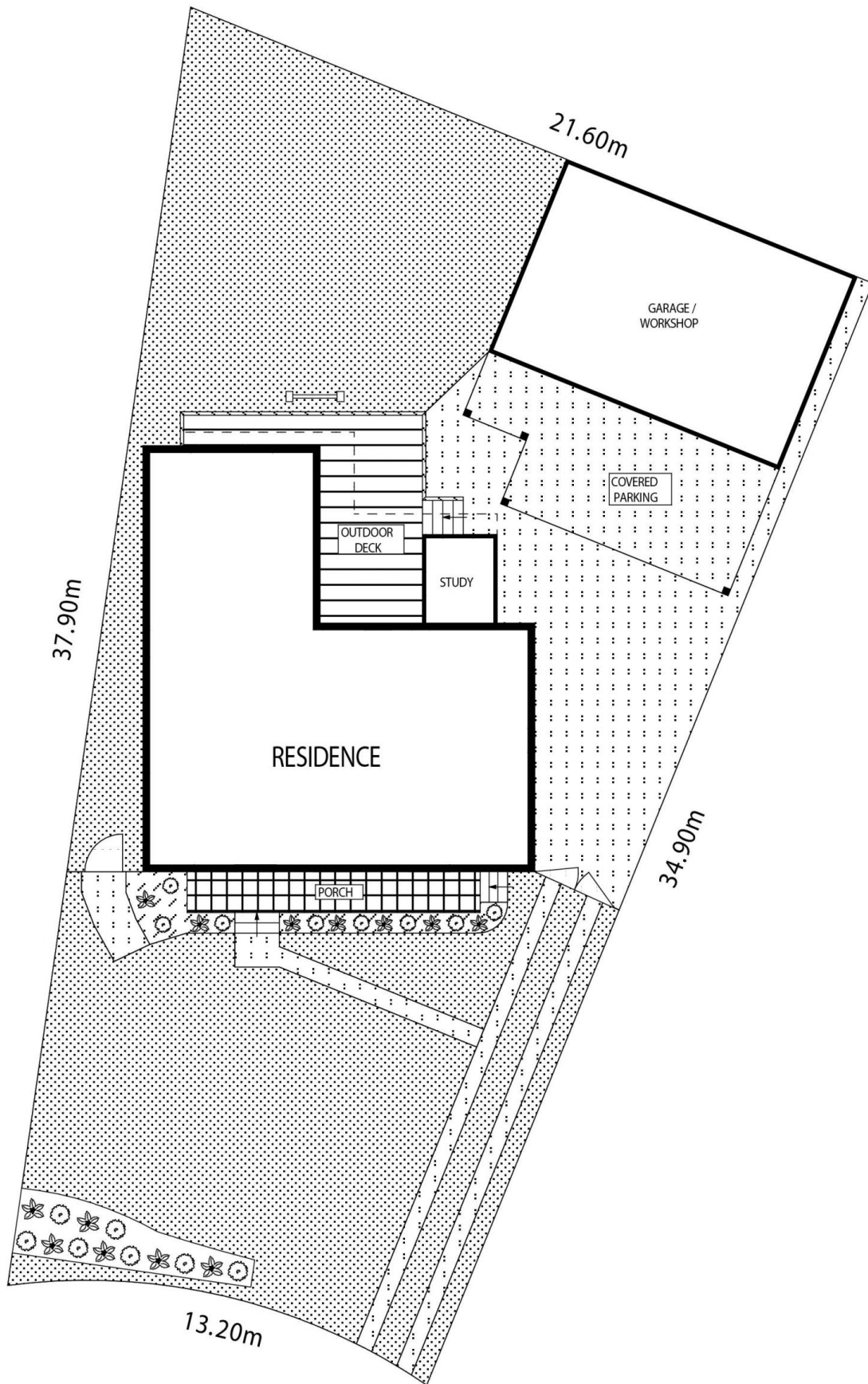
SITE PLAN
